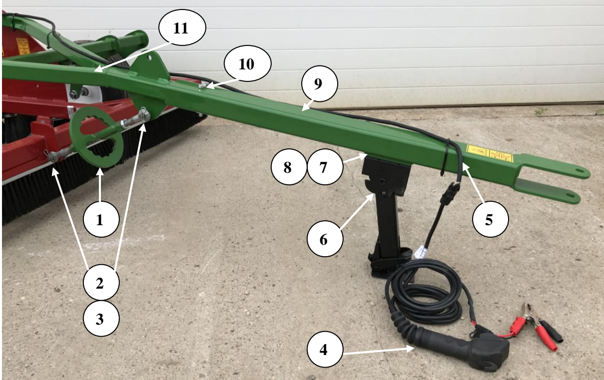
Figure 2: Hitch, Electrical
