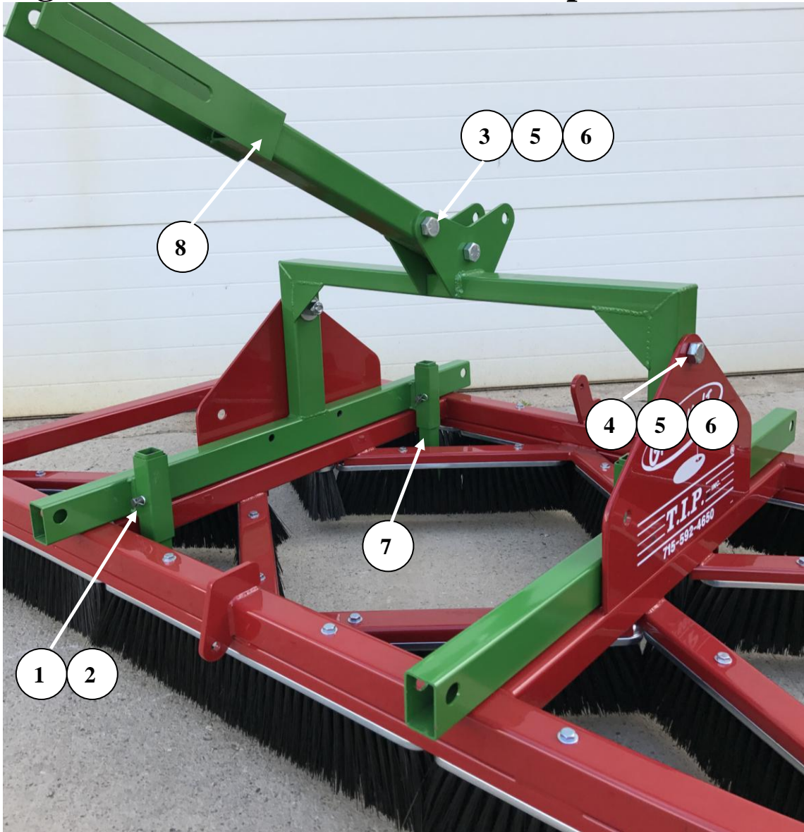
Figure 5: Groom-It 3 PT Mount Option
